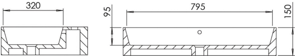
SECTION VIEWS
