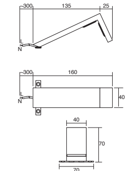
ARAL 3923 £109.20 W40 x D160 x H70 mm 2x1.2W • Transformer Included • IP21
