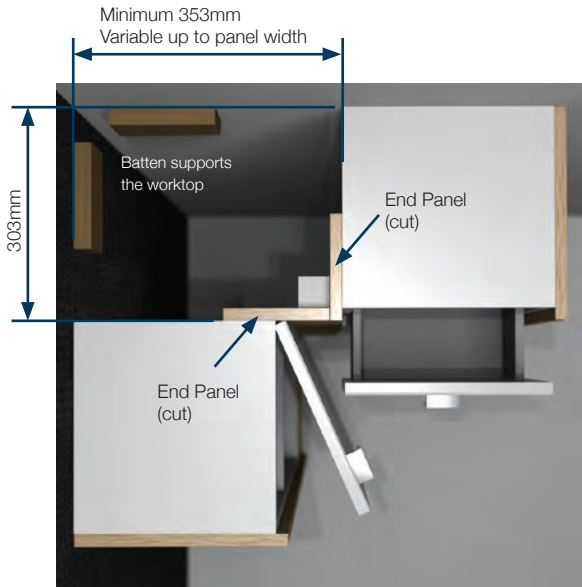
Layout 2: Variable. Suitable for drawers (Using end panels in corners).
